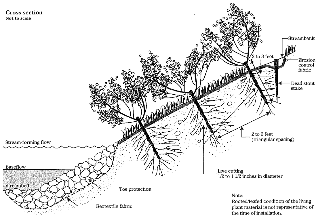
Figure 5 Live Staking 61
