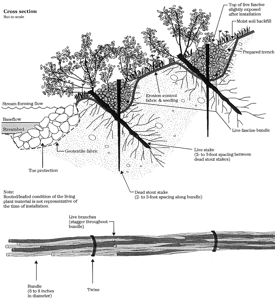
Figure 6 Live Fascines 62
