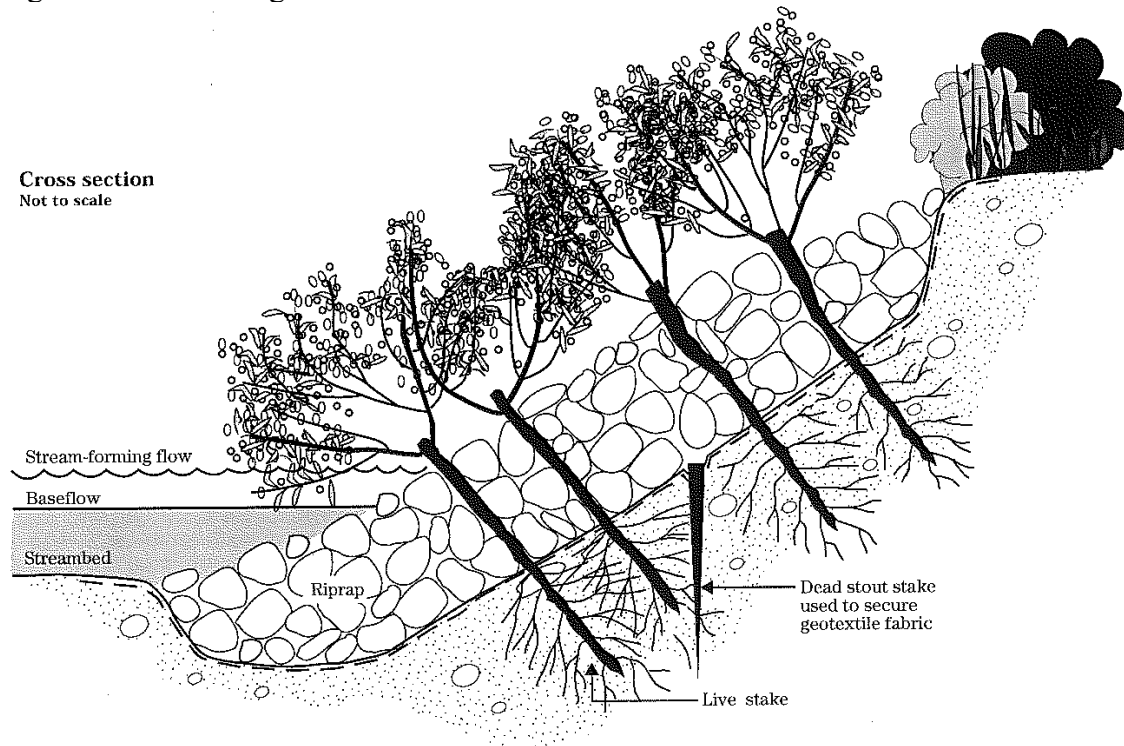
Figure7 Joint Planting
