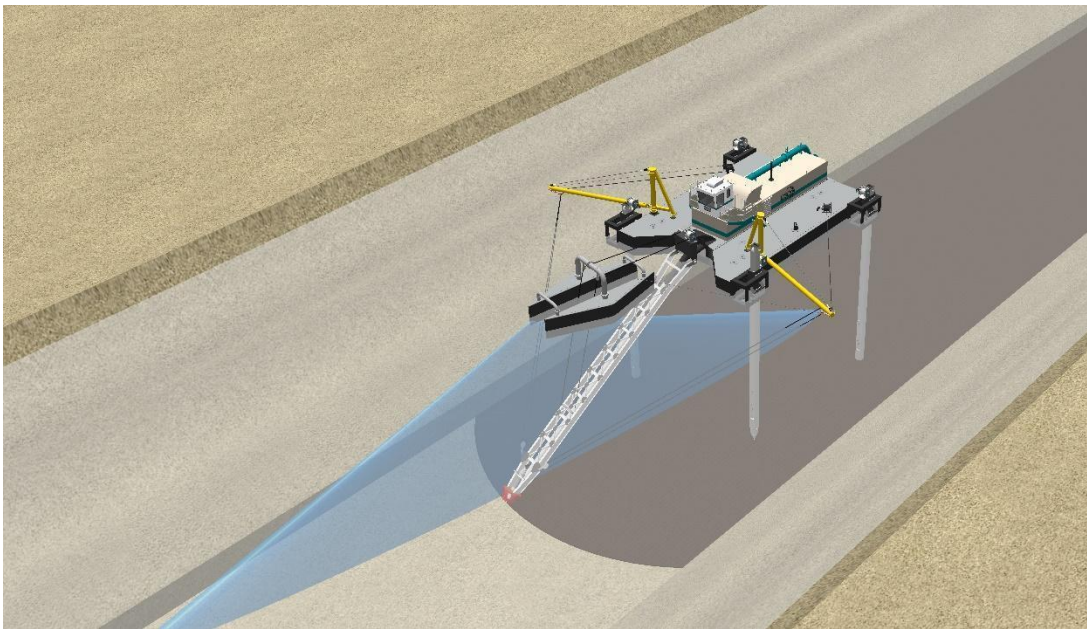
Figure 18 Illustration of a Hydraulic Dredge Using Multibeam Sonar Imaging
