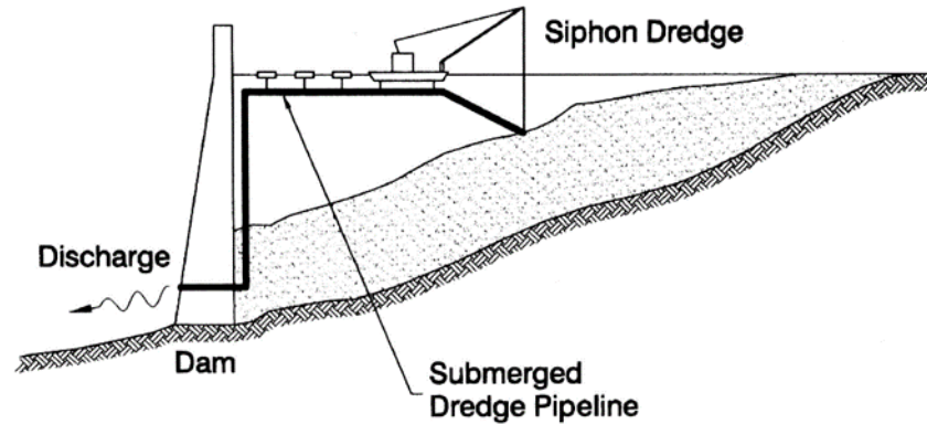
Figure 22 Differential Head Operating Principal of a Siphon Dredge
