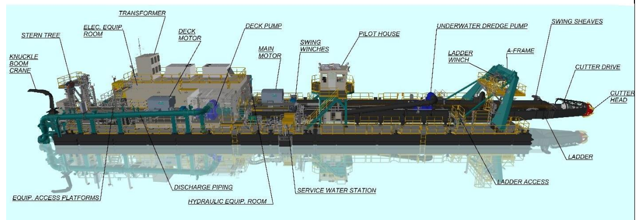
Figure 15 Dredge with Ladder-Supported Submersible Pump and Other Components
