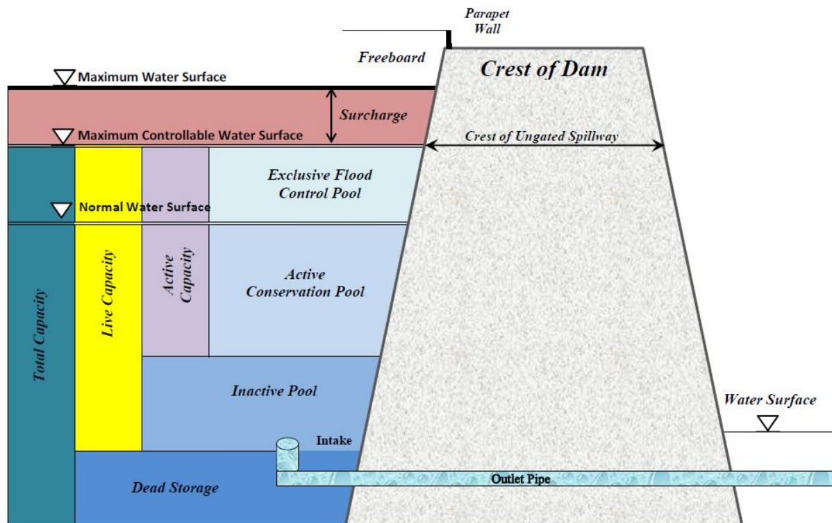
Figure 5 Reservoir Water Allocation Definitions
