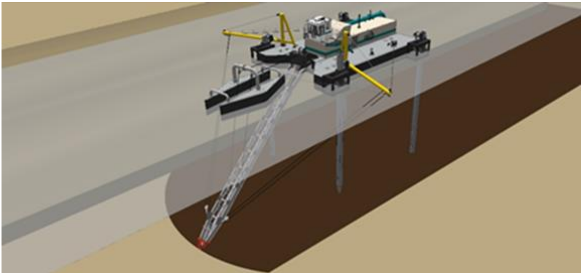
Figure 9 Swinging Ladder Cutterhead Suction Dredge
