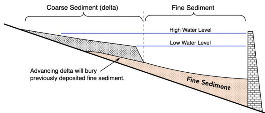
Figure 1 Longitudinal Pattern of Sediment Composition Typically Found in a Reservoir
