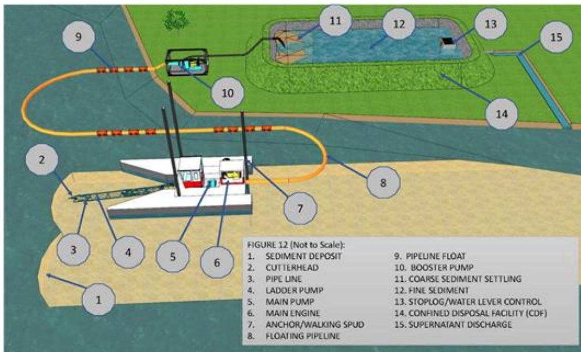
Figure 10 System Components of a Swinging Ladder Cutterhead Suction Dredge Depositing Slurry in a Confined Disposal Facility
