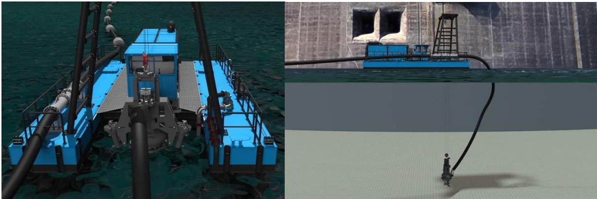
Figure 13 Hydraulic Dredging with Cable-Supported Submersible Pump
