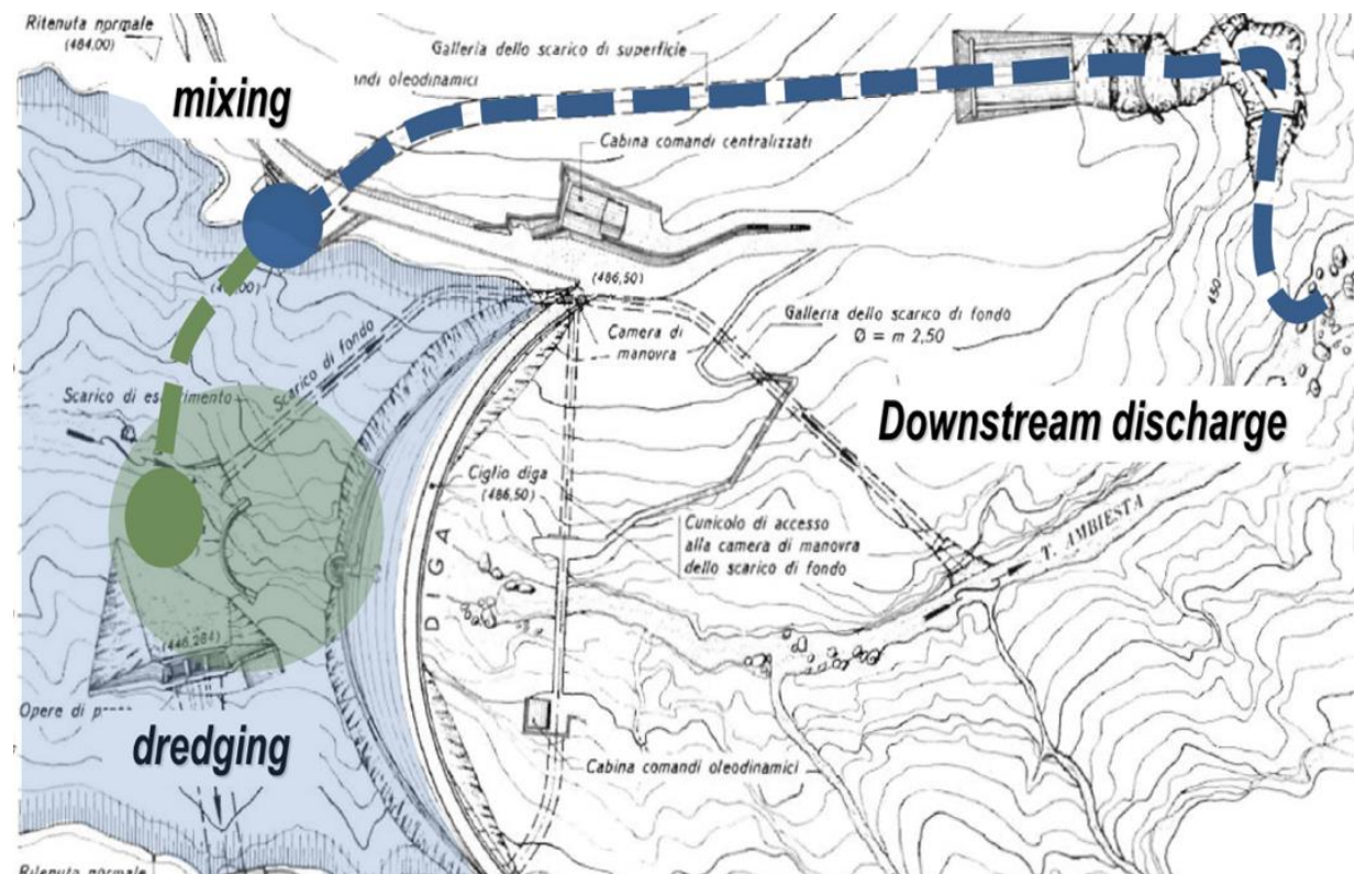
Figure 20 Ambiesta Dam Dredging Concept
